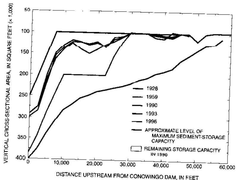
Figure 4. Changes in vertical cross-sectional area for selected years and cross-sectional area at sediment-storage capacity in the Conowingo Reservoir. (From Langland and Hainly, 1997.)
